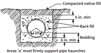
Figure 3. Proper bedding & backfilling
