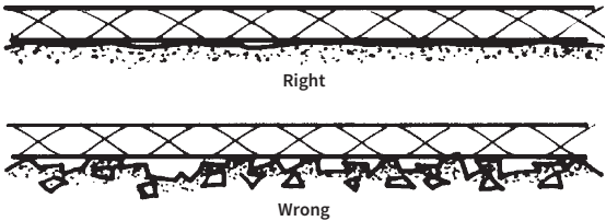
Figure 2. Proper trench bottom preparation
