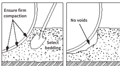
Figure 4. Proper Haunch Filling
