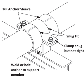
Figure 9. Pipe Anchor
