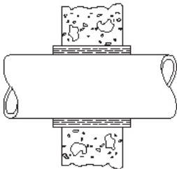
Figure 5. Wall penetration
